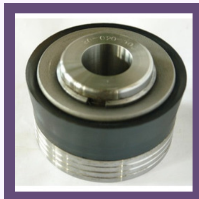
Mud Pump Piston Cup
